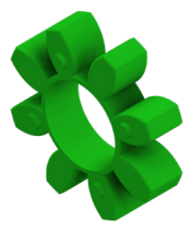
BLACK SPIDER 92-94Sh A THERMOPLASTIC YELLOW SPIDER 92-94Sh A POLYURETHAN RED SPIDER 96-98 Sh A POLYURETHAN GREEN SPIDER 64 Sh D POLYURETHAN
